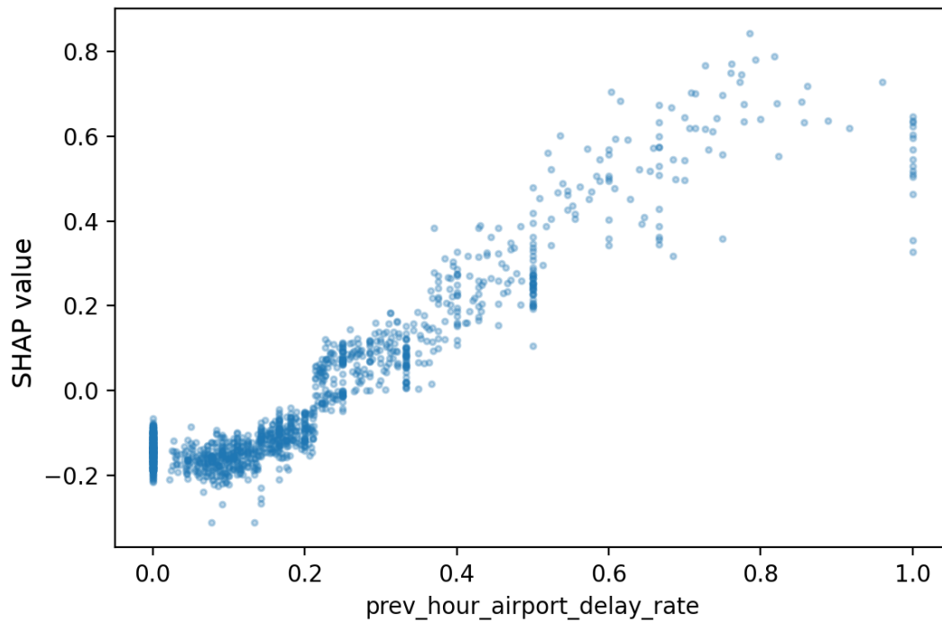
Figure 3. SHAP Dependence Plot for the Previous-Hour Airport Delay Rate
