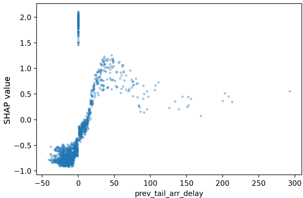
Figure 2. SHAP Dependence Plot for Previous-Flight Arrival Delay
