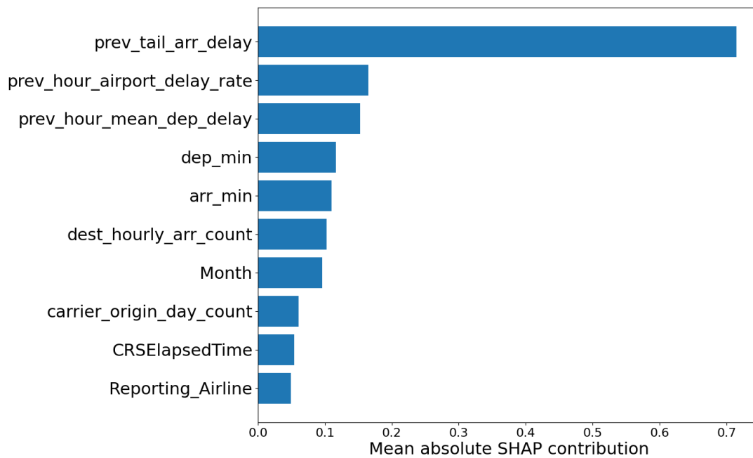
Figure 1. SHAP Summary Plot for the Operational XGBoost Model
